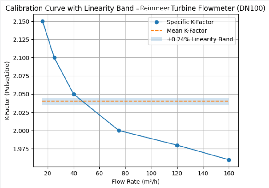
Calibration Curve and K-Factor Behavior
