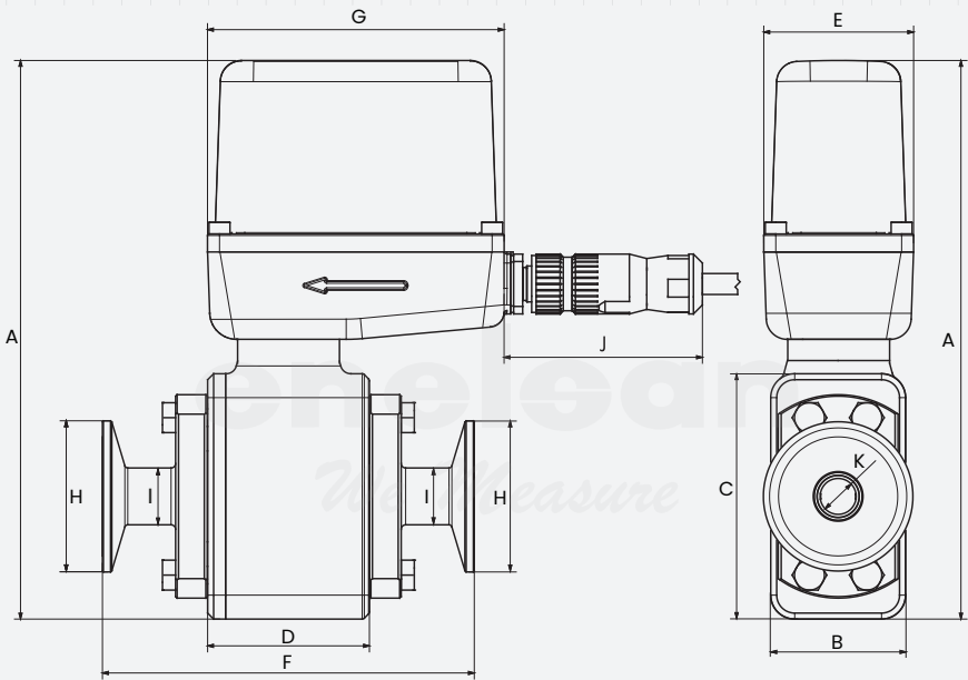
Emfil15 xx Dimensions (mm)
