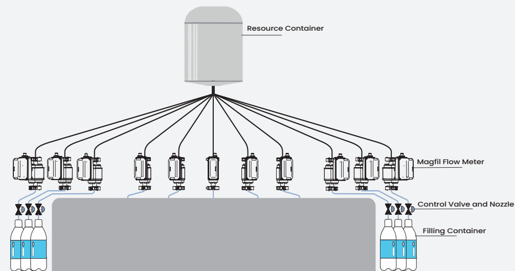
Installation on the rotary filling machine.
